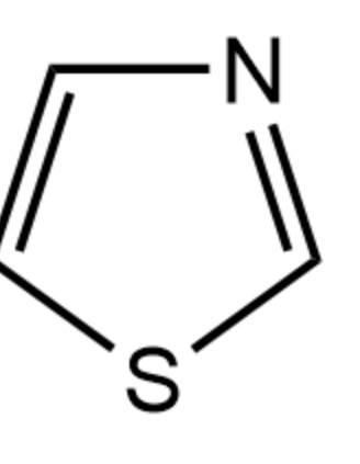
Thiazole 噻唑
