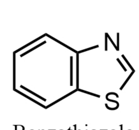
Benzothiazole 苯并噻唑
