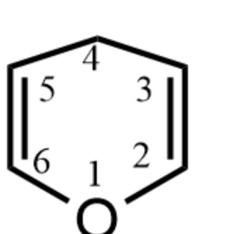
4H-Pyran 吡喃
