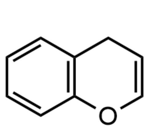
benzopyran 苯并吡喃
