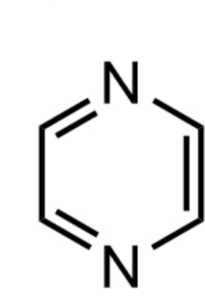
Pyrazine 吡嗪
