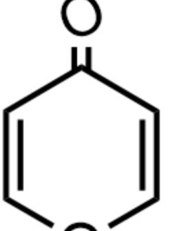
Gamma-pyranone 伽马-吡喃酮
