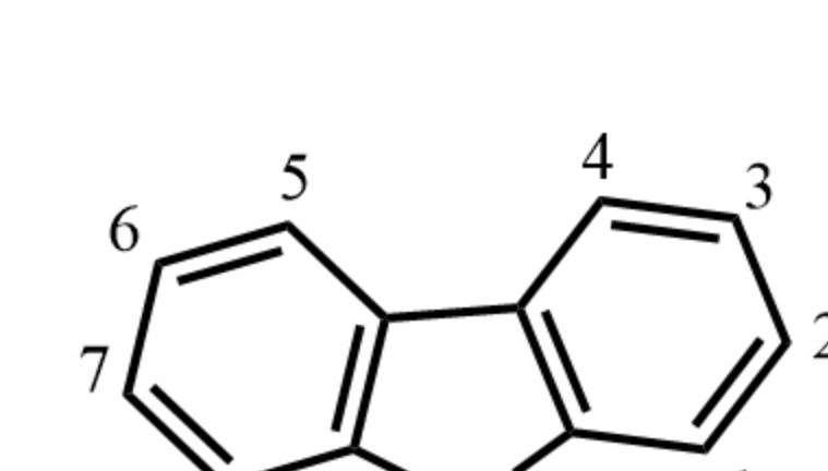
Carbazole, 咔唑
