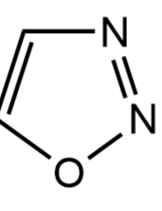
1,2,3-Oxadiazole 恶二唑
