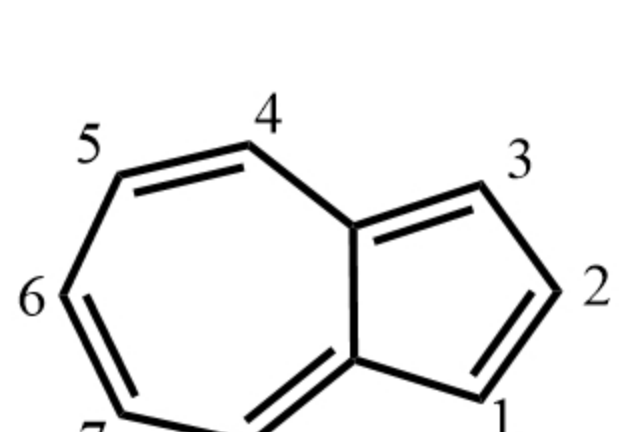
Azulene 甘菊蓝
