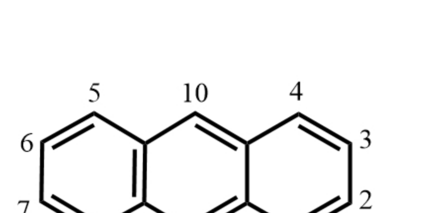
Anthracene, 蒽 / 并三苯
