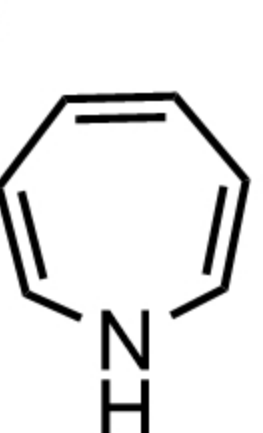
azepines 1H-氮杂莰
