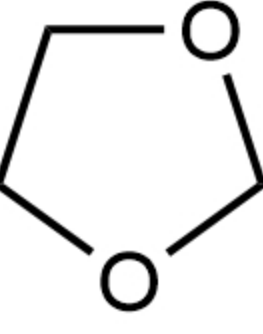
1,3-Dioxolane 1,3-二氧戊烷
