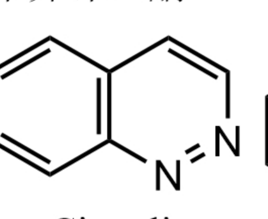
Cinnoline 噌啉
