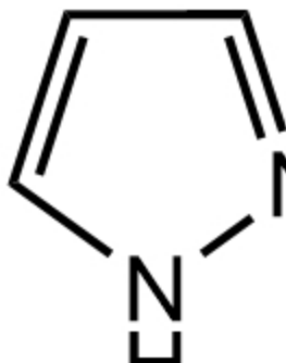
Pyrazole 吡唑
