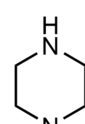
Piperazine 哌嗪
