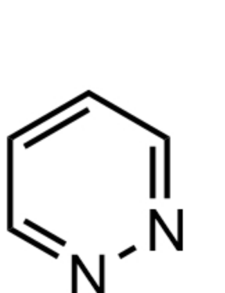
Pyridazine 哒嗪
