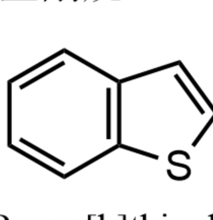
Benzo[b]thiophene 苯并噻吩
