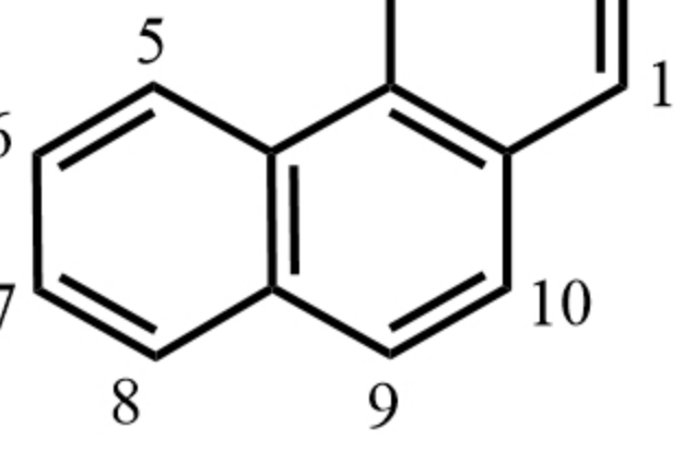
Phenanthrene, 菲
