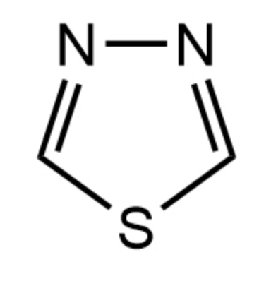
1,3,4-Thiadiazole 噻重氮/噻二唑
