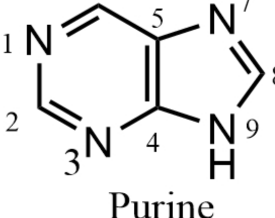
Purine 嘌呤
