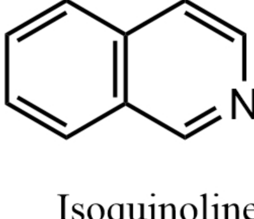
Isoquinoline 异喹啉
