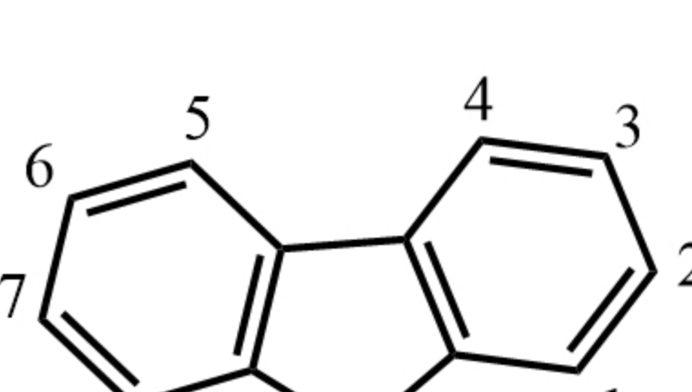
Fluorene 芴
