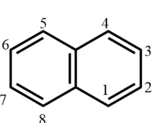
Naphthalene 萘
