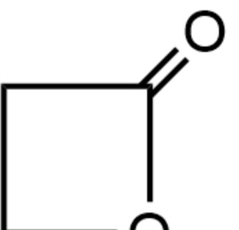
Beta propanolactone Beta-丙内酯
