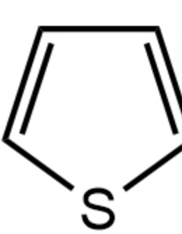
Thiophene 噻吩
